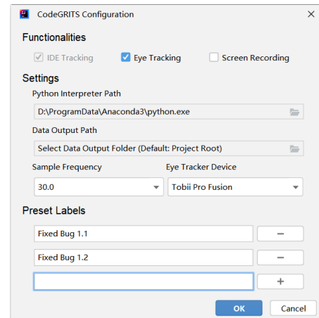
Figure 2: Configuration panel of CodeGRITS.
