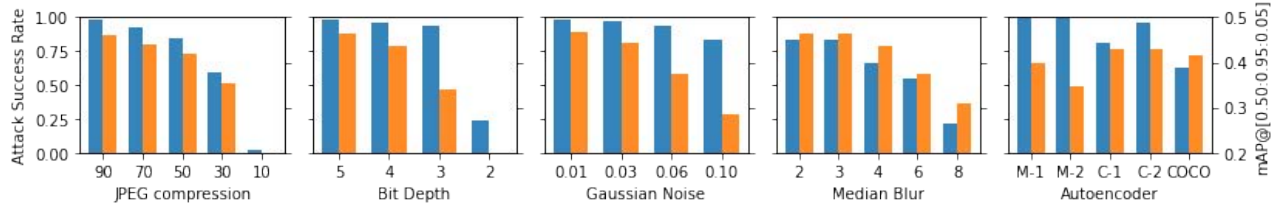
Figure 12: ASRs (blue bars) and mAPs in benign scenarios (orange bars) with the input-transformed defenses. The x-axis represents the strength of defenses for all defenses except the denoise autoencoders. The character of 'M' and 'C' denotes the MNIST and CIFAR-10, respectively, as the training dataset of autoencoders. The number '1' and '2' denotes the two different model architecture proposed in [27].
