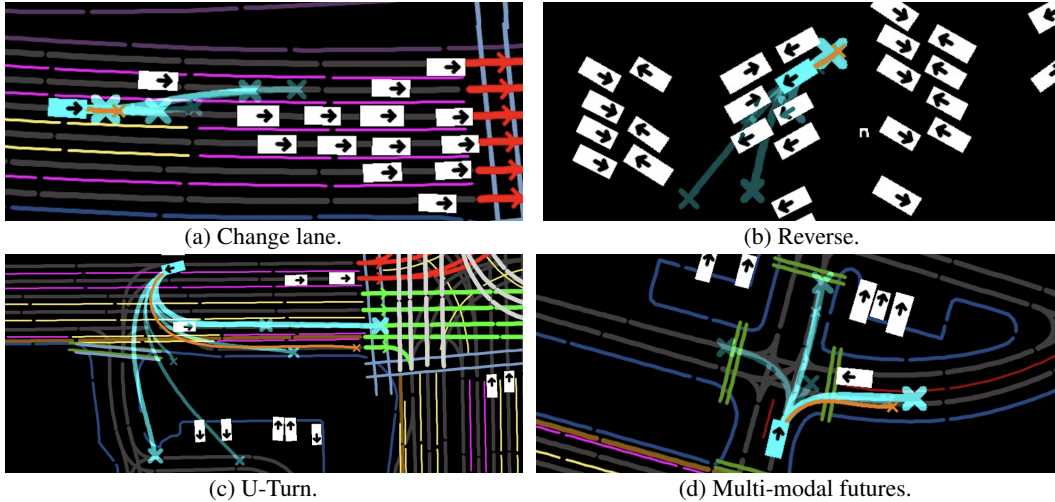
Figure 9: Qualitative results of HPTR predicting vehicles . Scenarios are selected from the WOMD validation dataset. The ground truth is in orange. The target agent and the predictions are in cyan. The most confident prediction has the least transparent color, the thickest line and the biggest cross.
