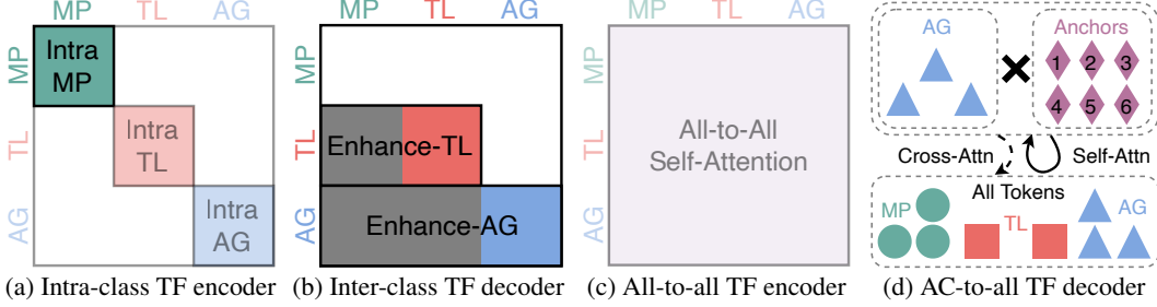
Figure 3: The hierarchical architecture of HPTR. Transformers are applied in sequential order from left to right, top to down. Some attentions are redundant and can be skipped for better efficiency. We propose the lower triangular attention matrix, which excludes the intra-TL, intra-AG and all-to-all self-attentions (the transparent parts). By removing the redundant attentions, this specific lower triangular architecture enables asynchronous token update during online inference. TF: Transformer. Attn: Attention. MP: Map. TL: Traffic lights. AG: Agents.
