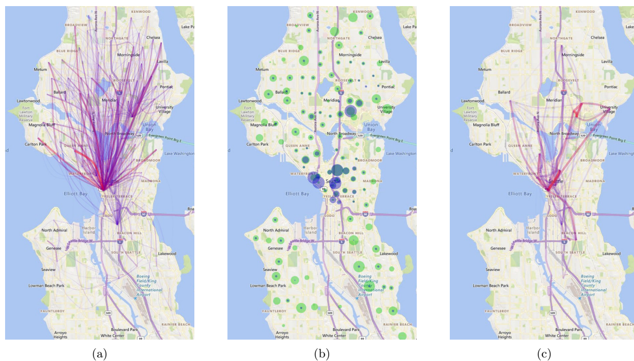
FIG. 2: (a): Average travels between census tracts of Seattle. (b): Population density; the green disks represent census tract populations and blue disks represent census tract population densities. (c): Top 20 census tracts with highest travels.
