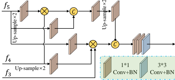
Fig. 3. Paralleled partial decoder is utilized to generate the global map.
