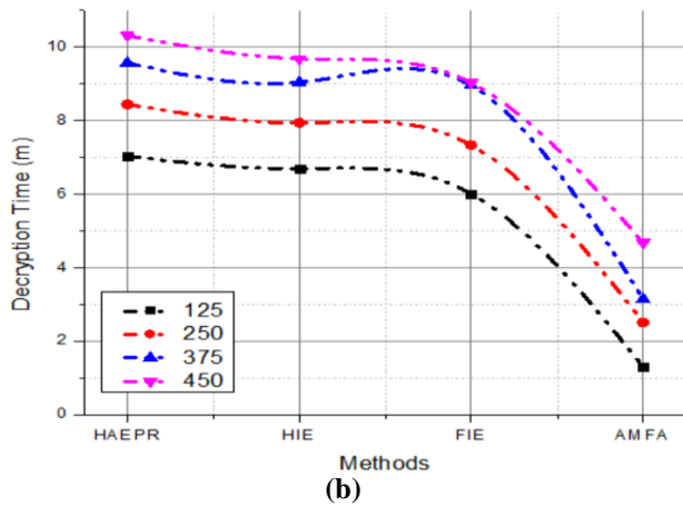
Figure 2: (a) encryption time and (b) decryption time
