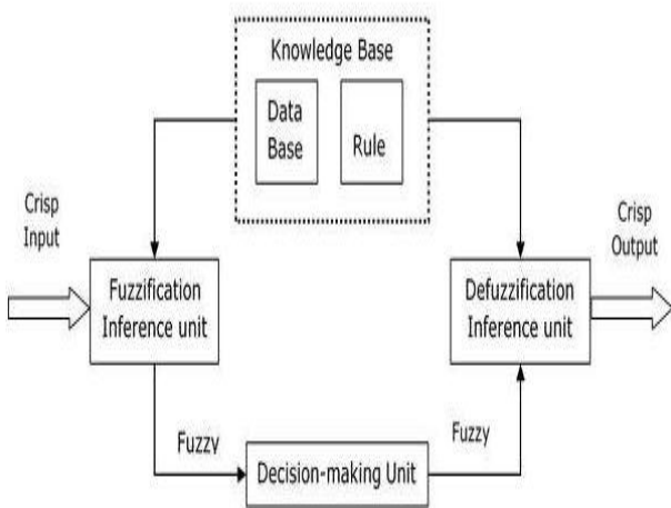
Fig 1.Fuzzy Inference System
