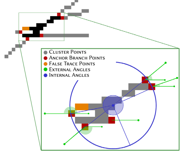
Fig. 3. Example of a cluster: cluster points (in gray), anchor points (in red), false trace points (in orange), external angle directions (in green), and internal angle directions (in blue).
