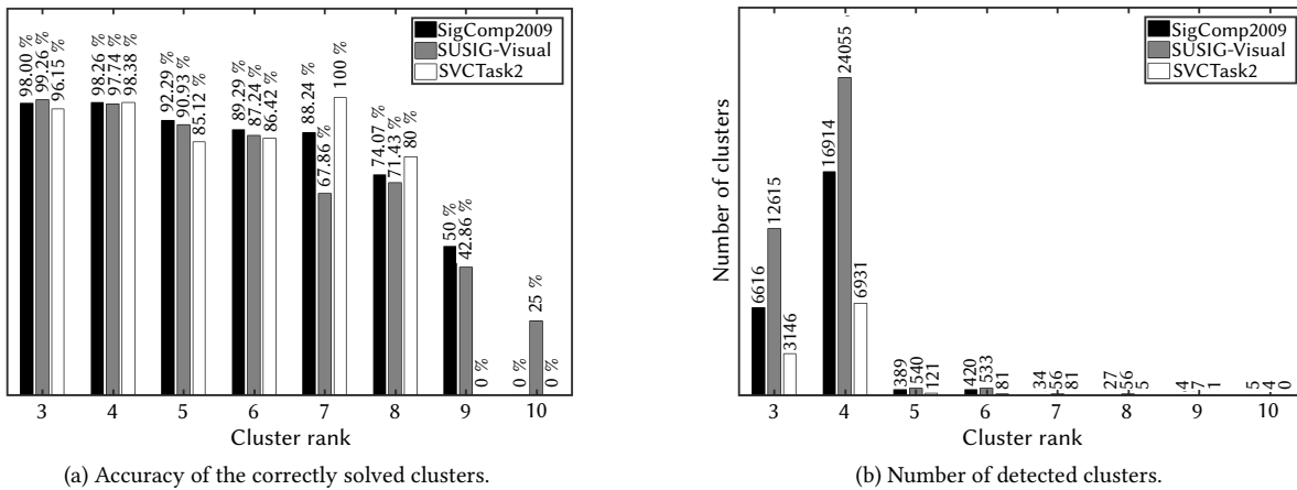
Fig. 9. Performance of the system solving the clusters found in each database.
