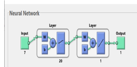
Fig. 15. Neural Network
