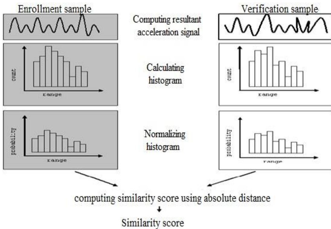
Figure 45: Applying the histogram similarity method on the acceleration signal
