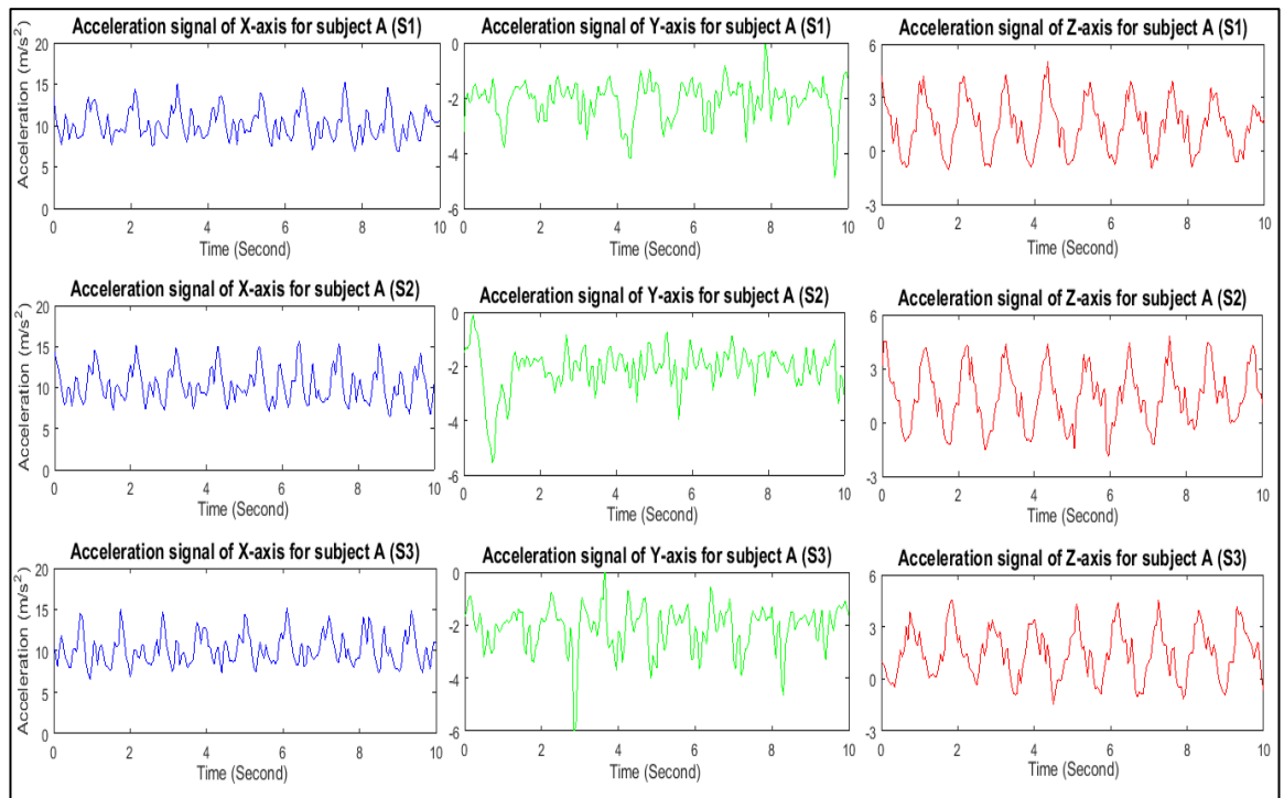
Figure 16: Three acceleration gait samples of three axes for Subject A
