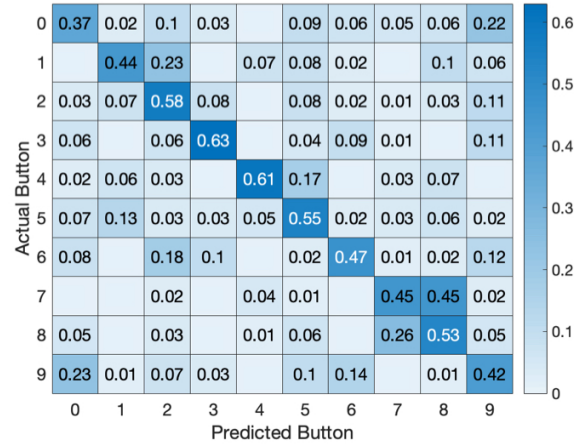
Figure 9: Breakdown of actual and predicted button classifications for the Galaxy Nexus when trained with one user’s data. An entry on row i and column j corresponds to button i being classified as j .
