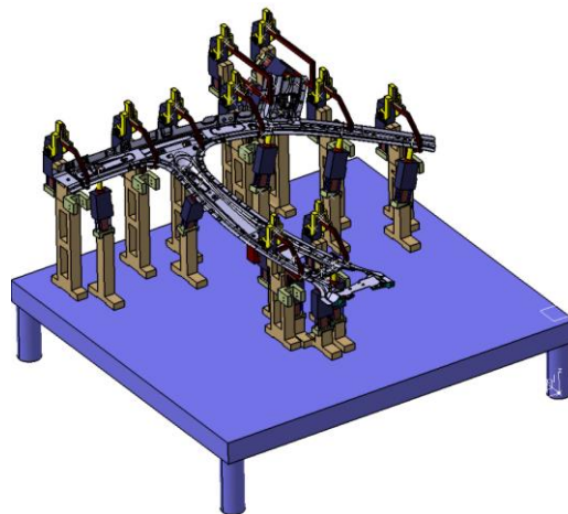
Figure 5. Design automation result - Isometric view
