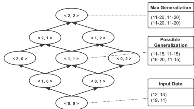
Fig. 4. An example lattice with level 2 for two attributes.
