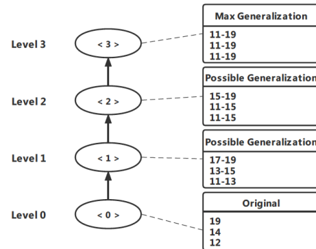
Fig. 3. An example lattice with level 2 for one attribute.
