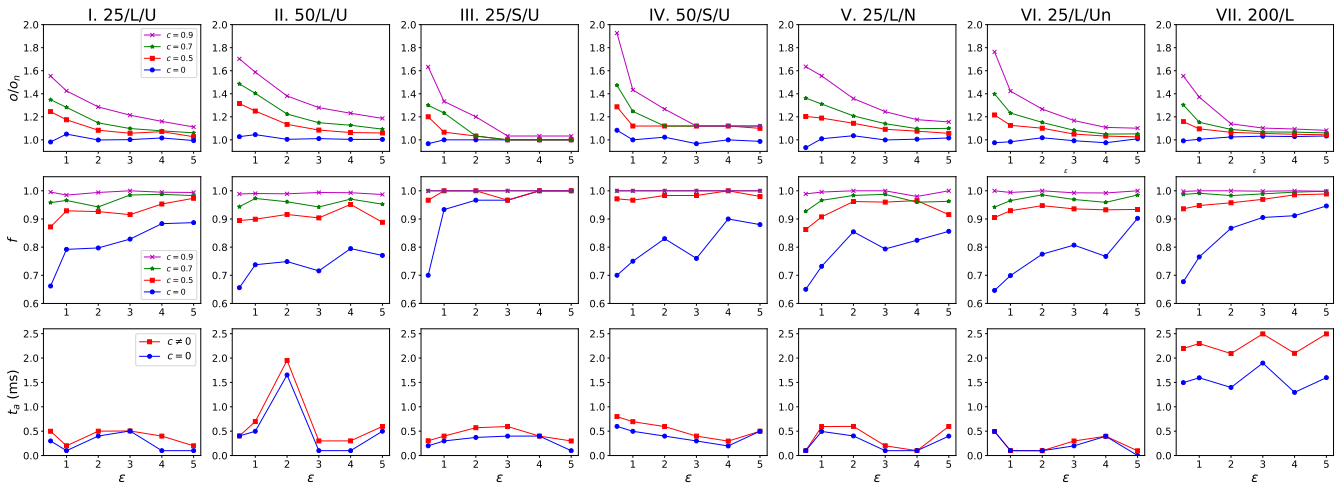
Fig. 6. The performance of the differential privacy with clustering method with different confidence factor c . The x-axis is \epsilon , and the y-axis is: the objective ratio o/o_n , the feasibility f , and the anonymization time t_a (ms).
