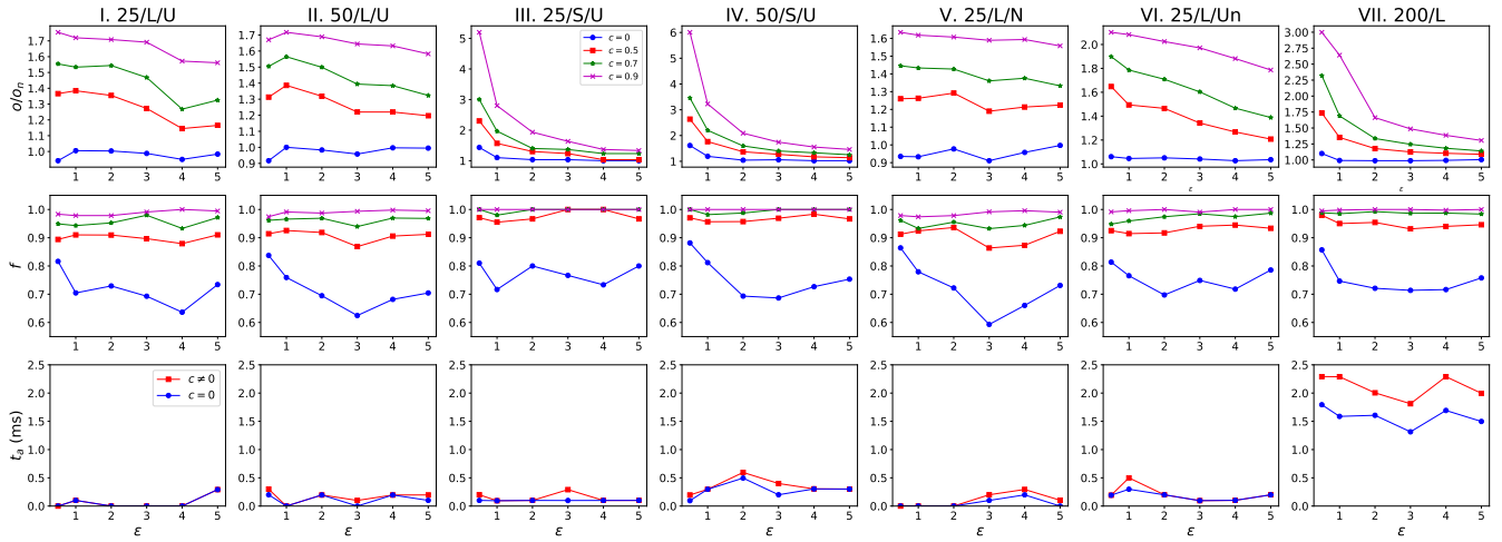
Fig. 7. The performance of the comparison method (differential privacy without clustering). The x-axis is \epsilon , and the y-axis is: the objective ratio o/o_n , the feasibility f , and the anonymization time t_a (ms).
