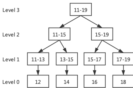
Fig. 2. An example full-domain generalization.
