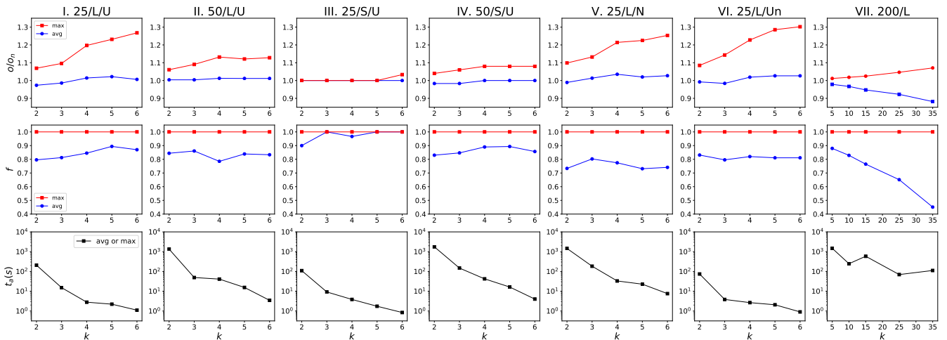
Fig. 8. The performance of the comparison method (k-Optimize with standard optimizer). The x-axis is k , and the y-axis is: the objective ratio o/o_n , the feasibility f , and the anonymization time t_a (s).
