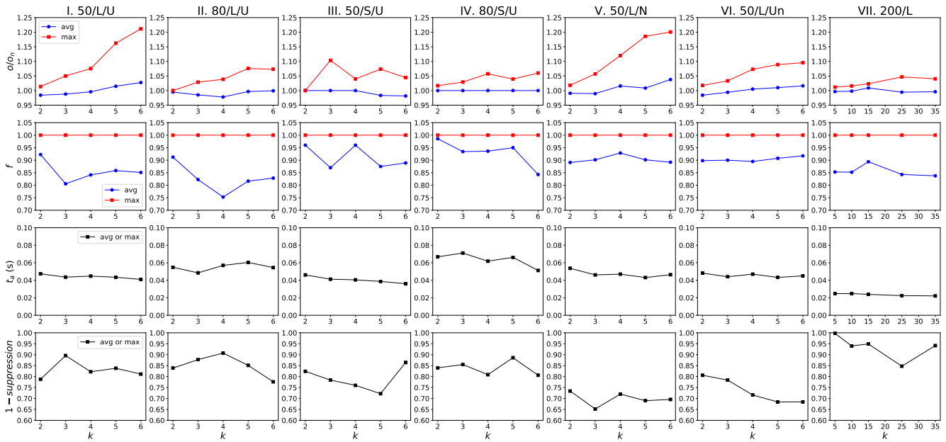
Fig. 5. The performance of the differential privacy with k -anonymity method using the average or the upper bound of intervals (with \epsilon' = 3 ). The x-axis is k , and the y-axis is: the objective ratio o/o_n , the feasibility f , the anonymization time t_a (s), and the proportion of the remaining data 1 - \text{suppression} .
