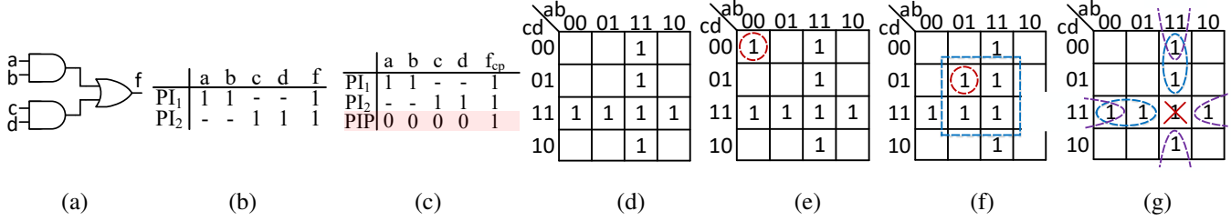
Figure 4: Logic optimization and logic locking: (a) The original circuit, (b) its PIT, (c) PIT of the corrupted circuit constructed by adding the PIP 0000, (d) K-map of the original circuit, (e) K-map of the corrupted circuit with the PIP 0000 as an isolated PI, (f) K-map of the corrupted circuit with the PIP 0101 leading to the creation of new PIs, and (g) K-map of with the removed PIP 1111 splitting the two original PIs.
