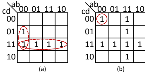
Figure 3: Logic synthesis using K-maps. a) The Boolean function f_1 is represented using only two PIs: cd and \overline{abd} . b) f_2 is represented using three PIs: abcd and \overline{abcd} .
