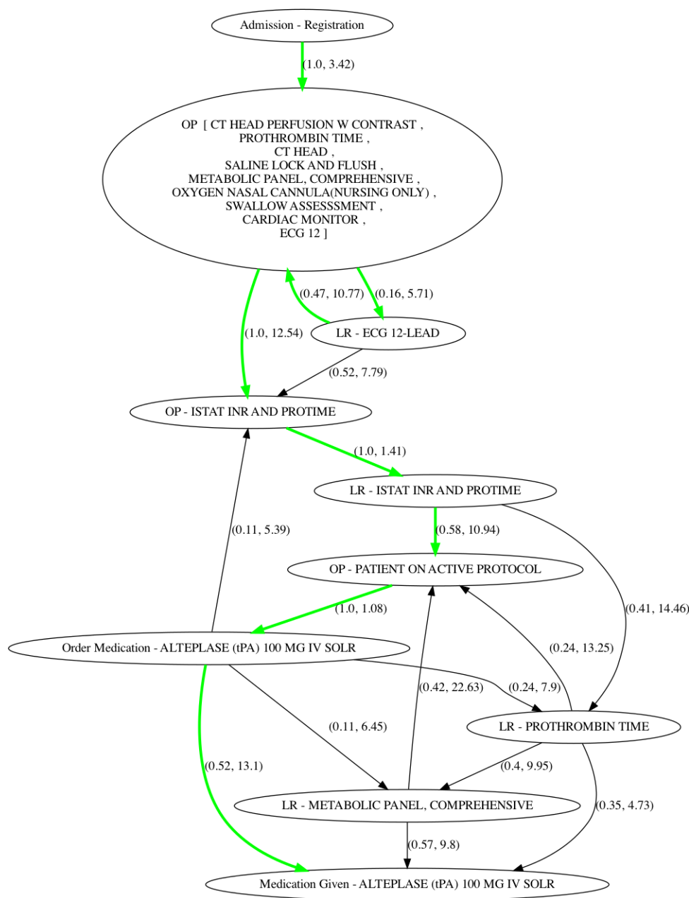
Figure 4: The process mining graph of the stroke patients with green path representing MCP; the path for the patient with the highest conformity score (0.64). The average conformity score for this cohort was measured as 0.36, which is within the expected range. Based on the definition of the average conformity score this means that each node has an average probability of about 0.36, which is in agreement with the fact that every node is connected to about 3 subsequent nodes for this graph.
