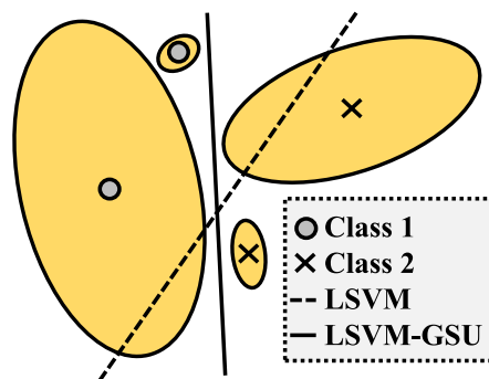
Fig. 21. A schematic view of SVM-GSU. Source: Reproduced based on [264].
