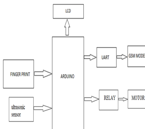
Fig. 1. Locker System Block diagram
