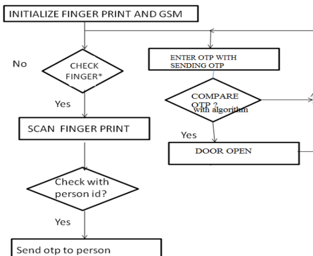
Fig. 10. Diagram of fingerprint-based security system
