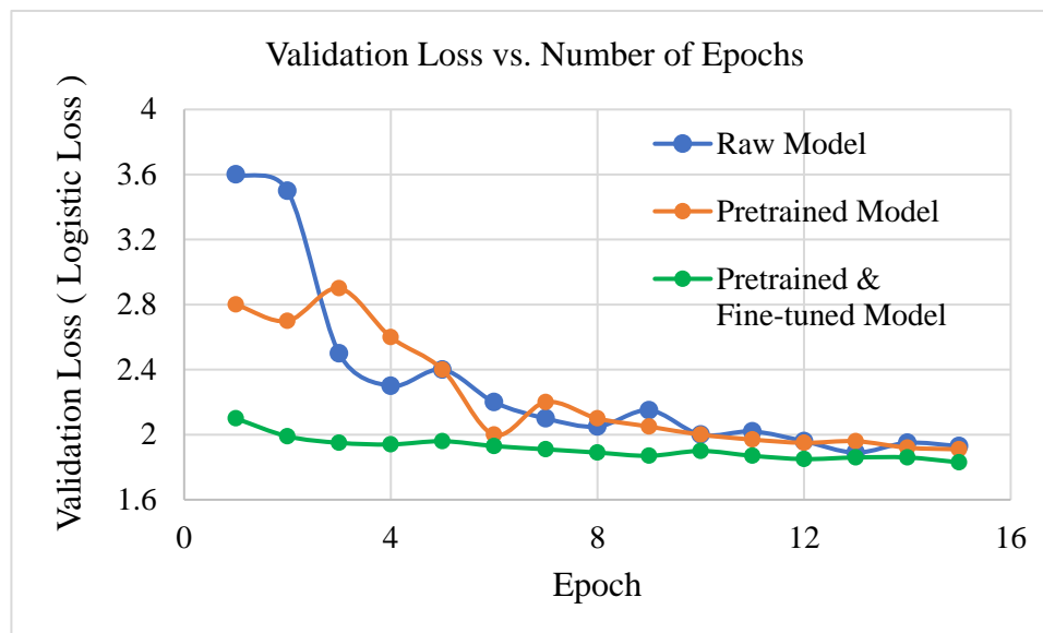
Figure 7 Validation loss progression of various models
