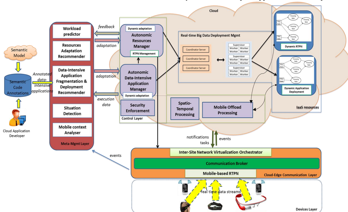
Figure 1: PrEstoCloud Conceptual Architecture
