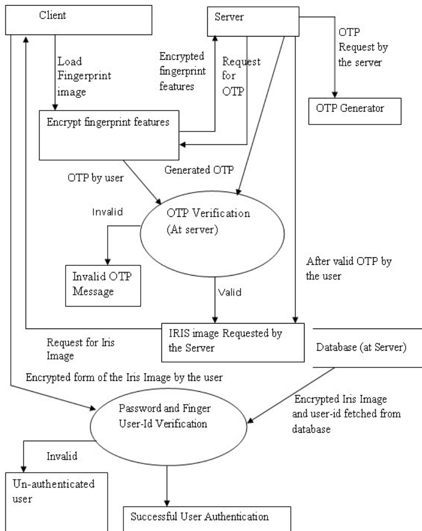
Fig.2: Dataflow Diagram of Proposed Multifactor Authentication
