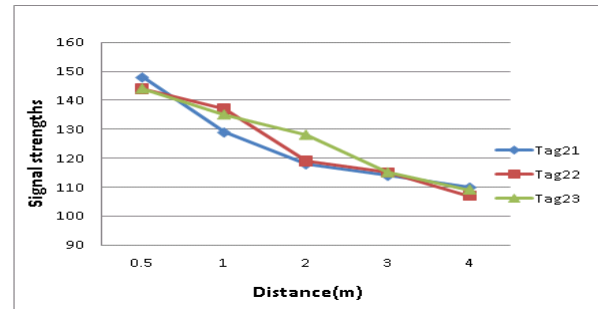
Fig. 9 Average value of filtered received signal strengths
