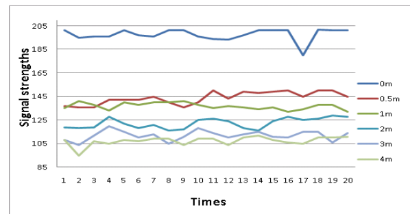
Fig. 8 Signal strength of Tag22 at different distances
