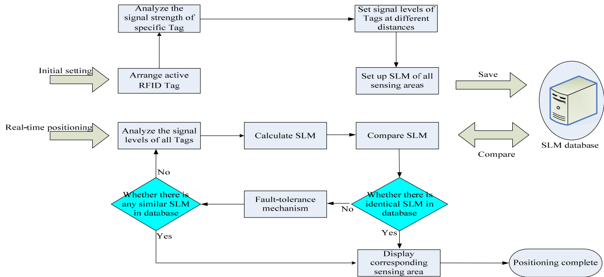
Fig. 2 Schematic diagram of positioning flow
