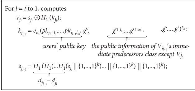
FIGURE 3: The process of key derivation.
