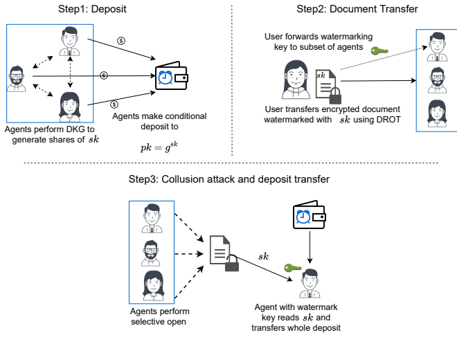
Fig. 1: Steps involved in the collusion deterrent escrow mechanism. Distributed key generation (DKG) is used by the agents to generate shares of secret key sk corresponding to public key pk . Distributed receiver oblivious transfer (DROT) is used by the user to transfer a copy of the document to the agents such that it contains the secret key sk as watermark.
