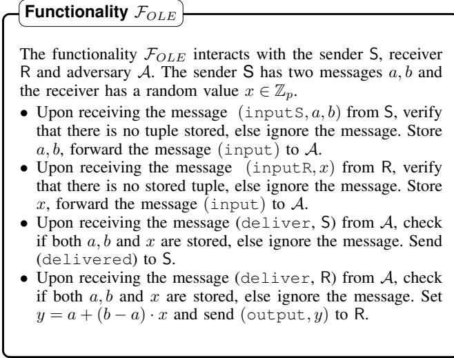
Fig. 4: Ideal Functionality Of the OLE protocol [35], [43]
