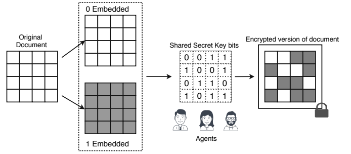
Fig. 2: Watermarking the document blocks and transferring them to the agents. Two versions of each block are obtained by watermarking 0, 1. The secret key bits are shared among the agents. Depending on the bit of the secret key, the transferred document block consists of the corresponding bit as the watermark. Thus final transferred encrypted document contains the whole secret key as the watermark.
