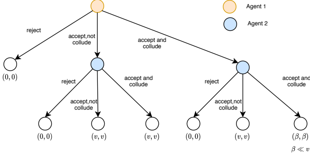
Fig. 7: Extensive form game induced by the user in CDE between two agents. v is the pay-off when agents do not collude and \beta \ll v is the pay-off when the agents collude
