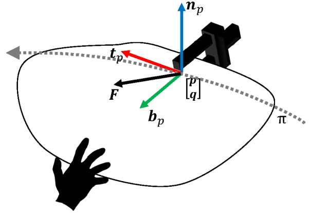
Fig. 1. The spatial part of collaborative policy \pi describes the motion of the robot. Vector \mathbf{F} denotes forces exerted by the human co-worker expressed in the robot coordinate system. The Frenet-Serret frame is specified by the tangent \mathbf{t}_p , normal \mathbf{n}_p and binormal \mathbf{b}_p . Current robot pose consists of a positional vector \mathbf{p} and a quaternion \mathbf{q} defining orientation.
