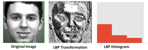
FIGURE 10: Figure shows the raw image at the left, the LBP version of the image is at the centre while the histogram of LBP image is at the right side.
