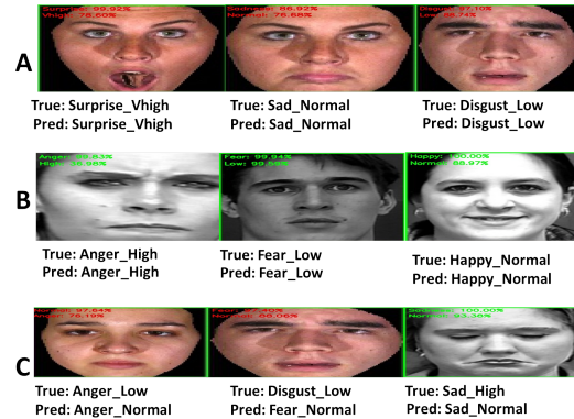
FIGURE 4: ML-CNN concurrent predictions of emotion with the associated intensity of BU-3DFE and CK+ test datasets. A and B are samples of correct predictions and C is the samples where one of either the emotion or the intensity is incorrectly predicted.
