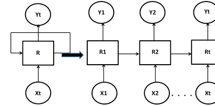
FIGURE 14: Figure showing the recursive operation of Recurrent Neural Network.
