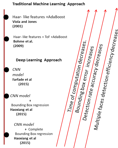
FIGURE 7: Analysis of some face detection algorithms.
