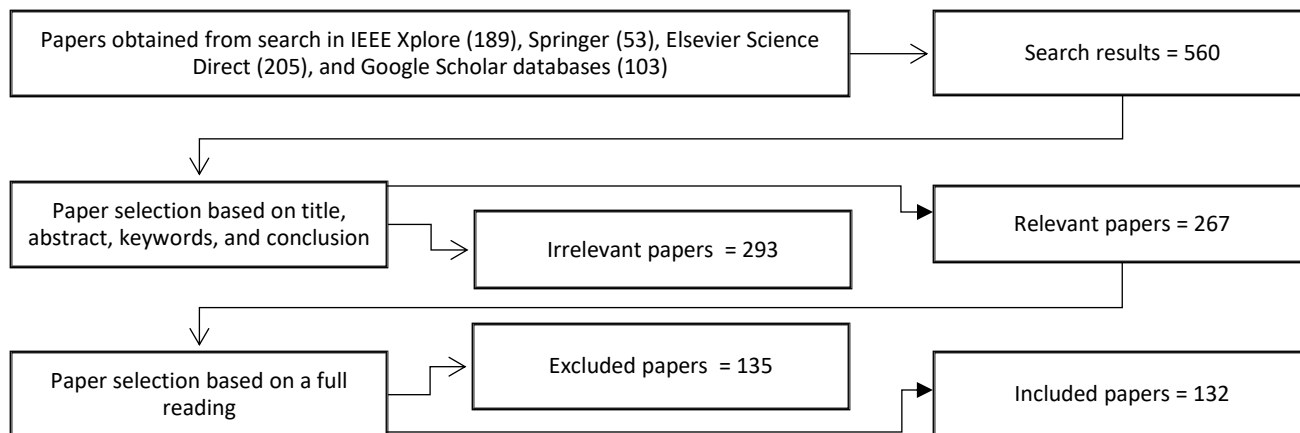
FIGURE 2. The inclusion/exclusion process
