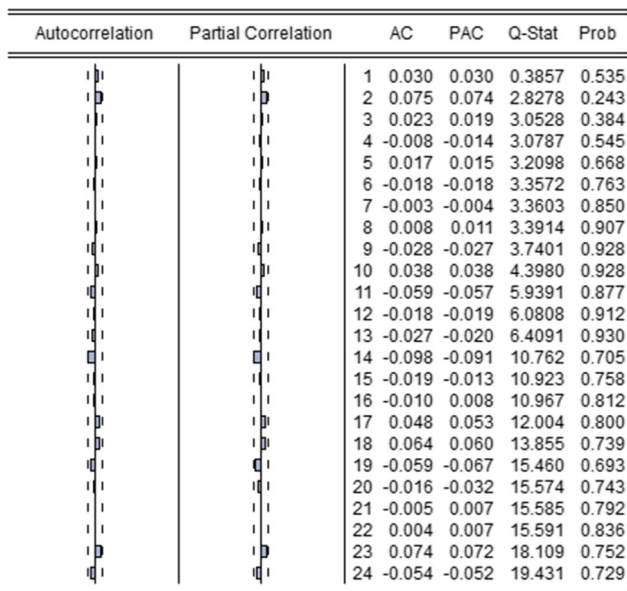
Fig. 7 Correlogram of closing price after differencing (DJI)
