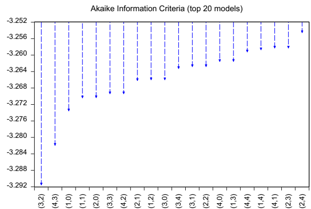
Fig. 14 Akaike information criteria (top 20 models)
