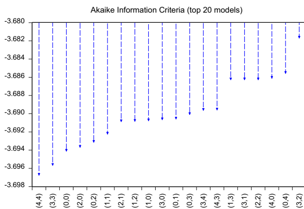
Fig. 13 Akaike information criteria (top 20 models)
