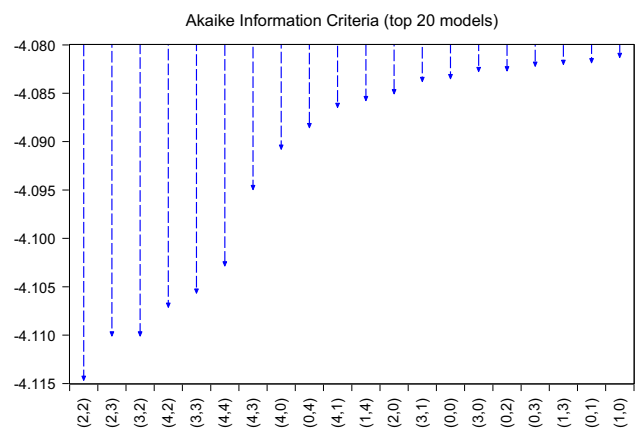
Fig. 15 Akaike information criteria (top 20 models)
