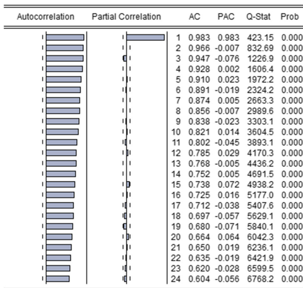
Fig. 6 Correlogram of closing price (DJI)
