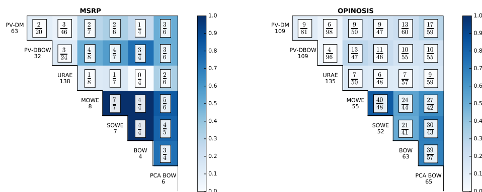
Figure 5.4: The misclassification agreement between each of the models for the MSRP (left) and Opinois (right) subcorpora. Below each model name is the total mistakes made. The denominator of each fraction is the number of test cases incorrectly classified by both models. The numerator is the portion of those misclassifications which were classified in the same (incorrect) way by both models. The shading is in-proportion to that fraction.
