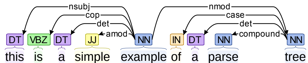
Figure 4.5: A dependency parse tree for the sentence This is a simple example of a parse tree , This flattened view may be misleading. example is at the peak of the tree, with direct children being: this, is, a, simple , and tree . tree has direct children being: of, a , and parse .
