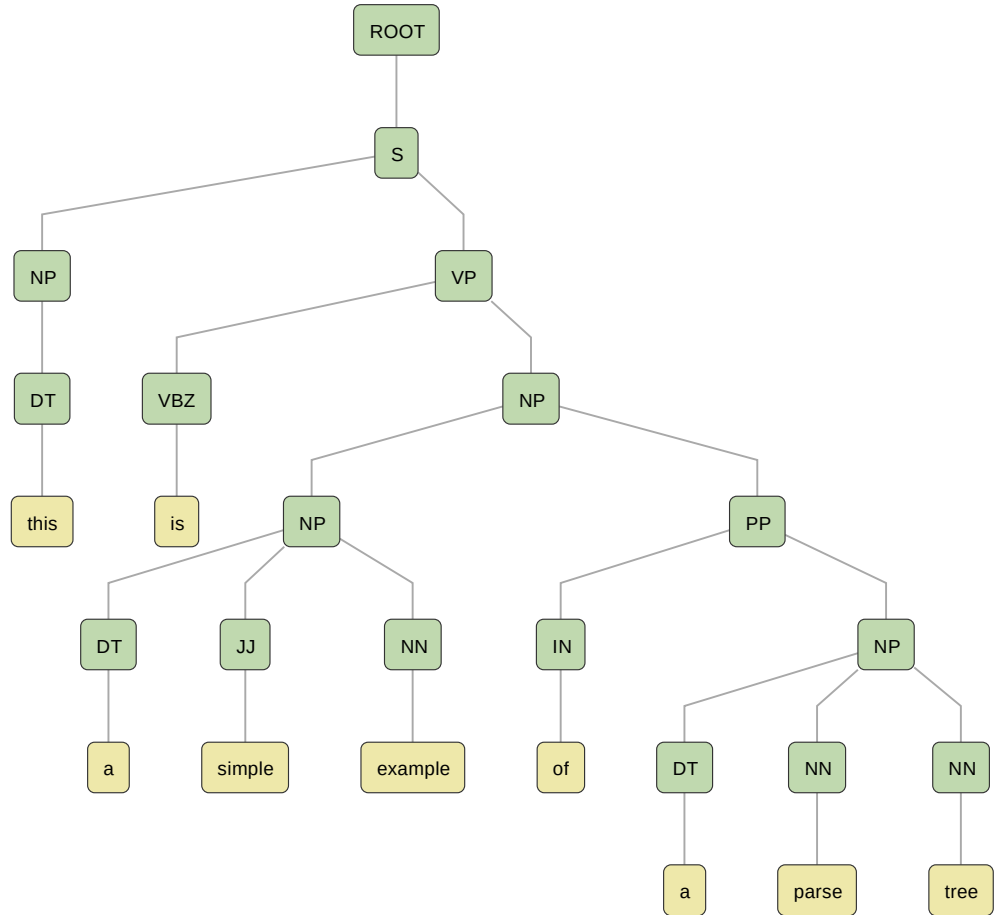
Figure 4.4: A constituency parse tree for the sentence: This is a simple example of a parse tree . In this diagram the leaf nodes are the input words, their immediate parents are their POS tags, and the other nodes with multiple children represent sub-phrases of the sentence, for example NP is a Noun Phrase.
