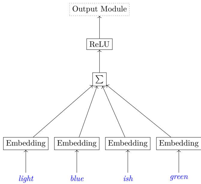
Figure 6.3: The SOWE input module for the example input light bluish green
