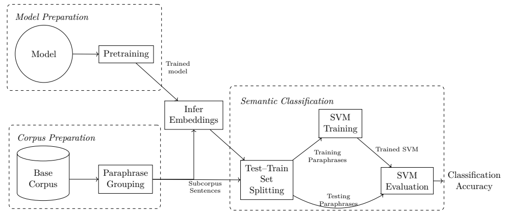
Figure 5.1: Process Diagram for the Evaluation of Semantic Consistency via our method
