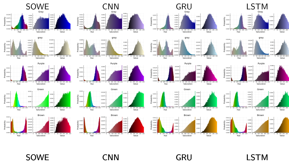
Figure 6.11: Some example distribution estimations for colors names which are completely outside the training data. The terms: Brown, gray, Gray, Green, and Purple, do not occur in any of the color data; however brown, grey green, and purple do occur.
