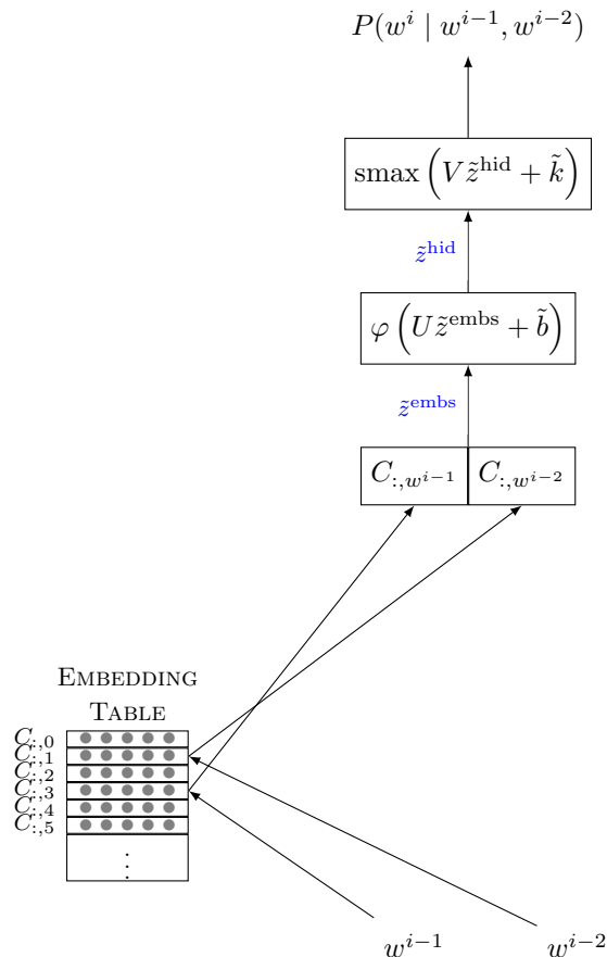
Figure 2.2: The Neural Trigram Language Model
