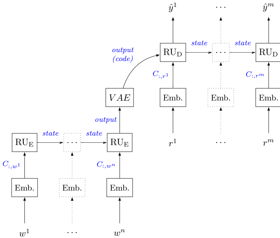
Figure 4.2: The VAE plus encoder-decoder of Bowman et al. (2016b). Note that during training, \hat{y}^i = w^i , as it is an autoencoder model. As is normal for encoder-decoders the prompts are the previous output (target during training, predicted during testing): r^i = y^{i-1} , with r^1 = y^0 = \langle \text{EOS} \rangle being a pseudo-token marker for the end of the string. The Emb. step represents the embedding table lookup. In the diagrams for Chapter 2 we showed this as a table but just as a block here for conciseness.
