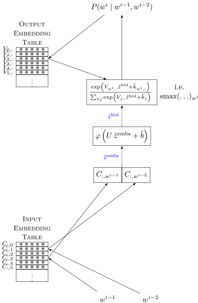
Figure 2.3: Neural Trigram Language Model as considered with output embeddings. This is mathematically identical to Figure 2.2
