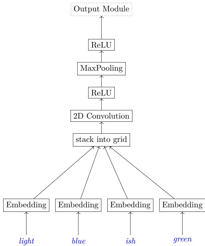
Figure 6.4: The CNN input module for the example input light bluish green .
