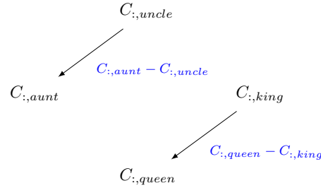
Figure 2.8: Example of analogy algebra
