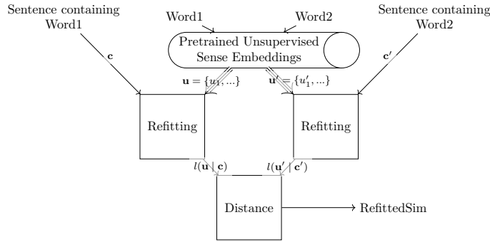
Figure 7.1: Block diagram for RefittedSim similarity measure
