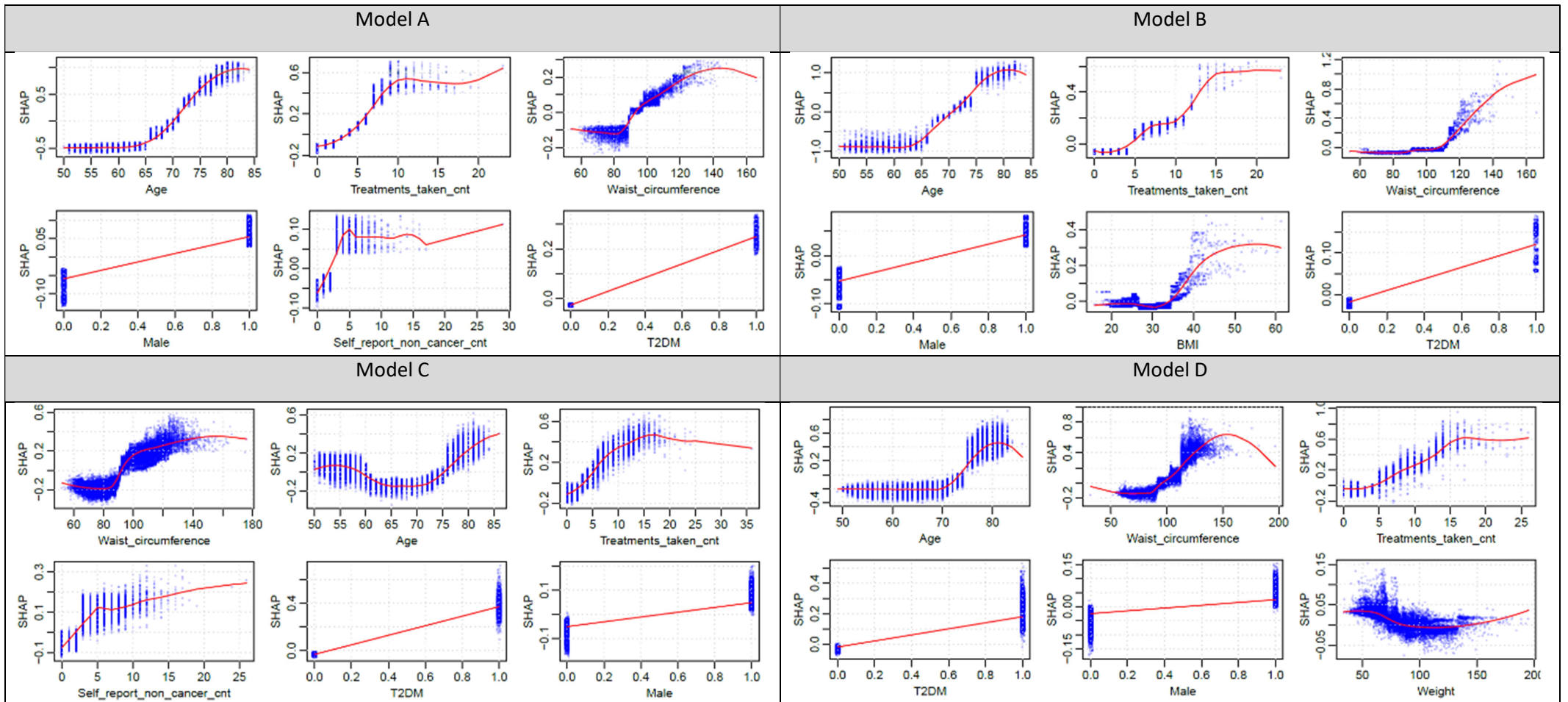
Figure 2. ShapVal dependence plots of top 6 risk factors ranked by mean \text{abs}(\text{shapley value}) (Lite model) for Models A, B, C, D respectively.
