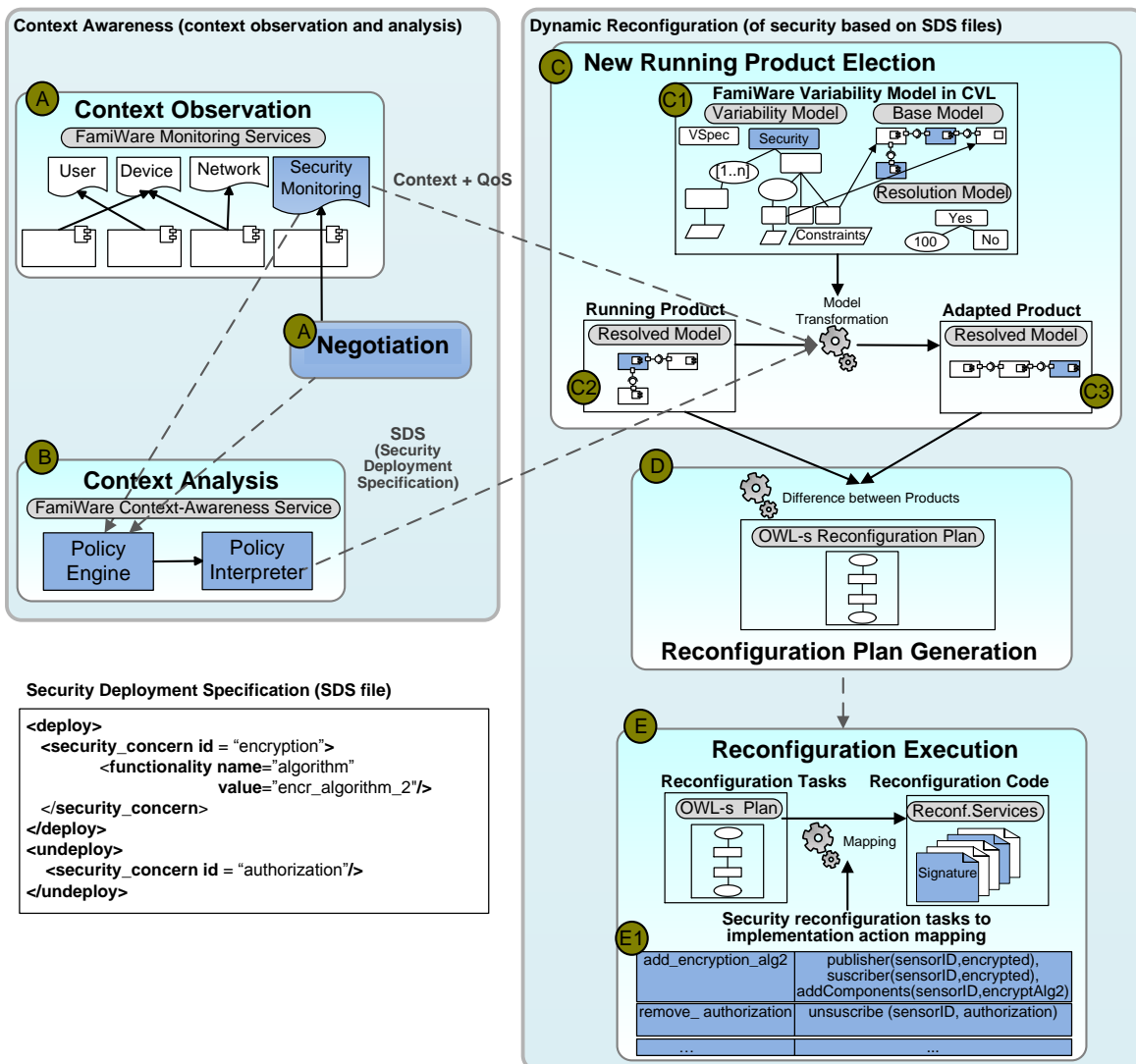
Figure 9. FamiWare runtime reconfiguration of security.
