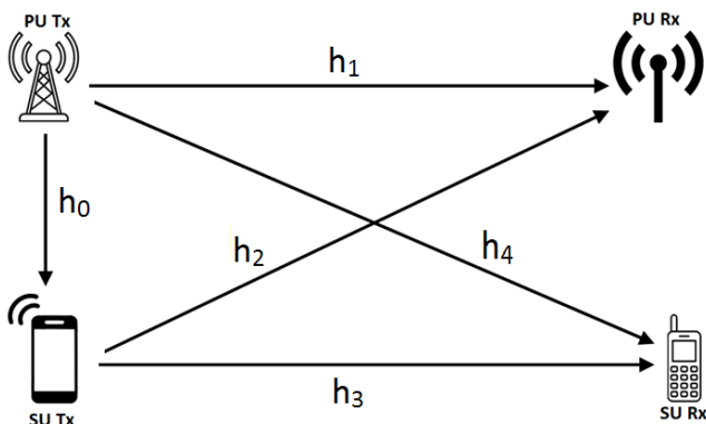
Fig.1. Relay assisted cooperative communication system in CR networks
