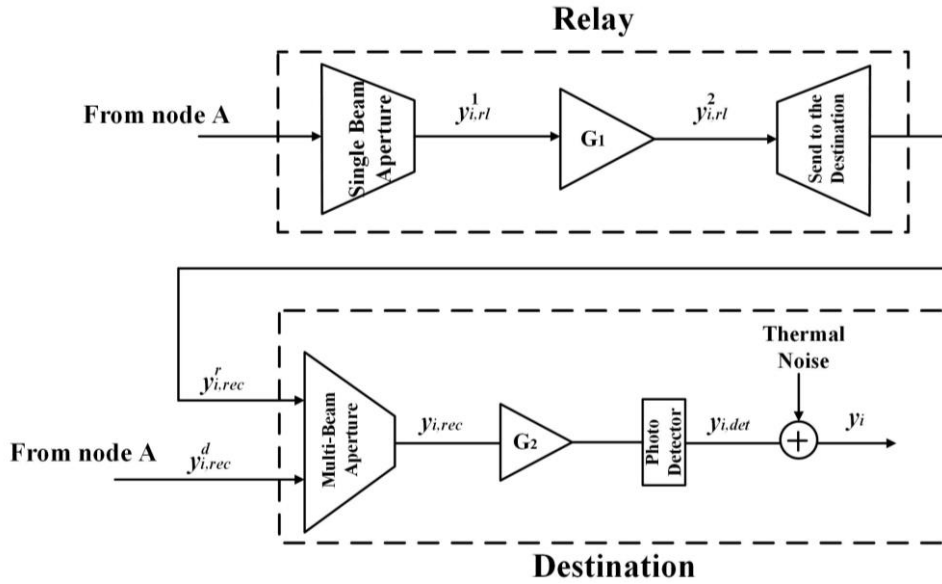
FIGURE 12. Block diagram of the receivers at the relay and the destination with the notations of the signals at different parts of the receivers [178].
