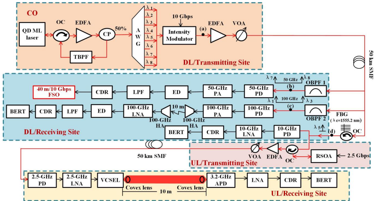
FIGURE 11. Experimental configuration of the proposed bidirectional WDM hybrid fiber-wired/fiber-wireless/fiber-IOWC/fiber-IOWC transmission system based on a self-injection locked quantum dash laser and a reflective semiconductor amplifier [177].
