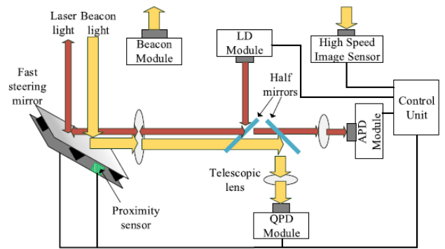
FIGURE 4. OOWC and HST communication [32], [68].
