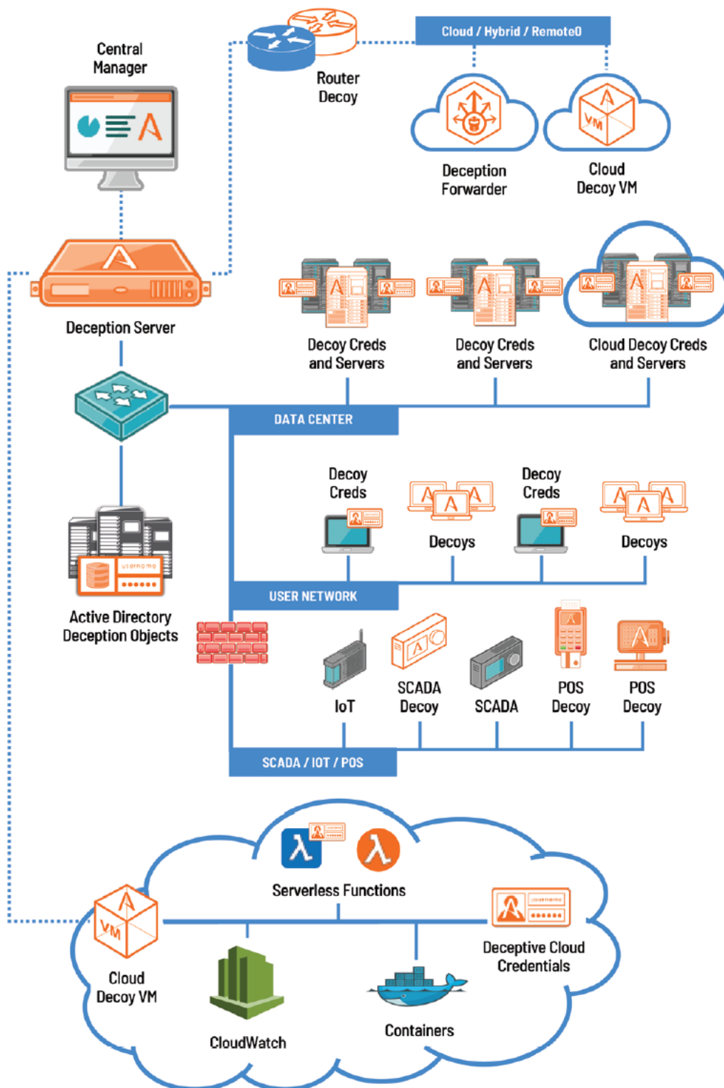
Figure 6. Typical Deception Deployment.
