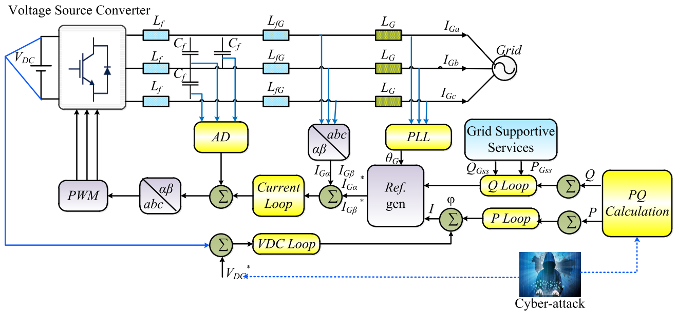
FIGURE 13. The P-Q control of grid-supportive voltage source converter: The black and blue lines signify the communication layer as well as attack elements injected into communication link/sensors, respectively.
