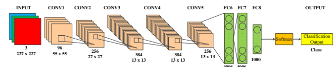
Fig. 2. Simplified illustration of AlexNet architecture
