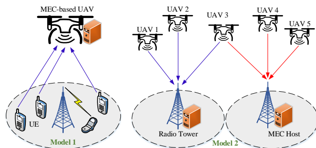
FIGURE 8: MEC-enabled UAV Networks Architecture.
