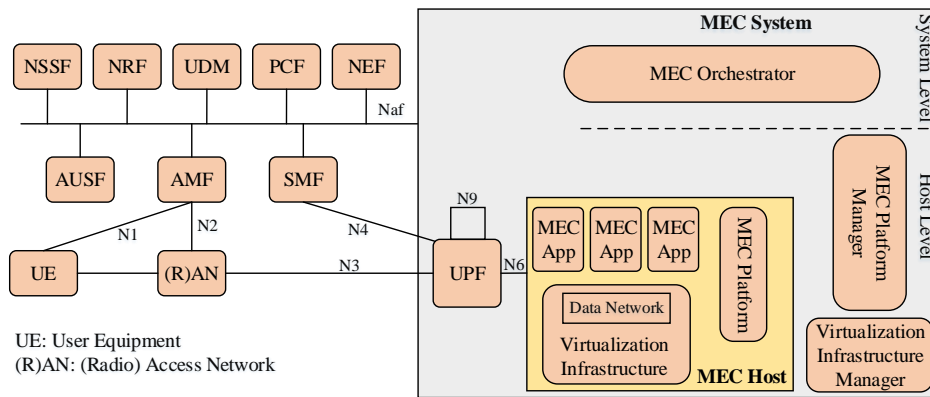
FIGURE 4: MEC integrated architecture in 5G [28].
