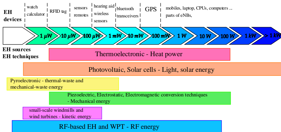
FIGURE 6: EH technologies with generated intermittent power and power consumption for various devices, adapted from [96]–[98].
