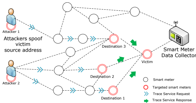
FIGURE 21: An attack scenario on the AMI [69].
