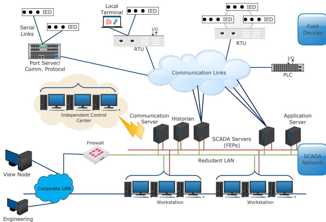
FIGURE 7: Power Grid's Supervisory control and data acquisition (SCADA) subsystem. https://eicoc.pnnl.gov/research/cybersecurity.stm .
