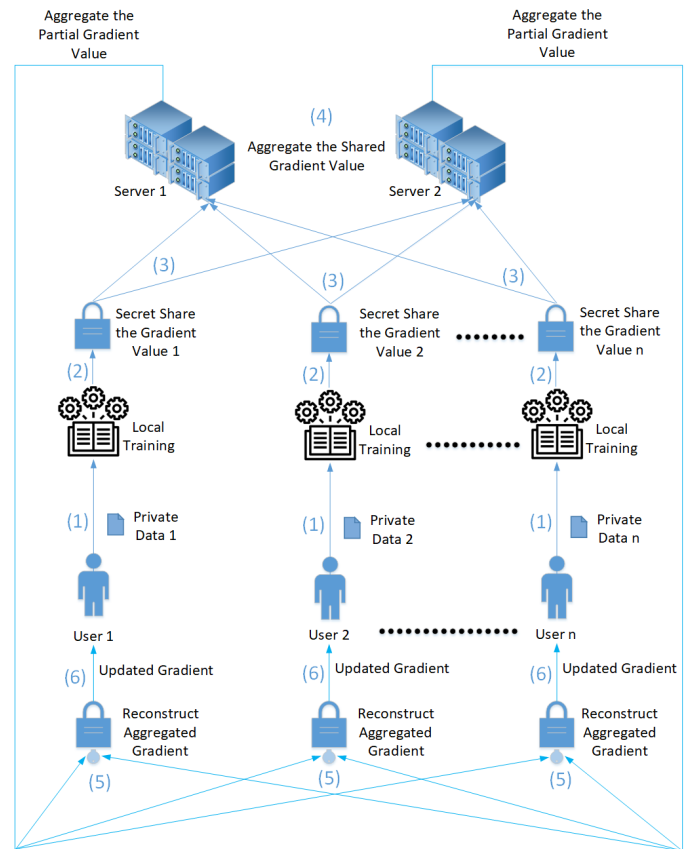
FIGURE 15. The Structure of Secure MPC-based PDDL
