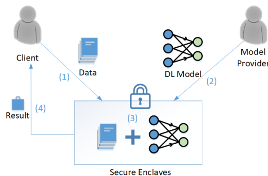
FIGURE 18. The Structure of Secure Enclaves-based PPDL
