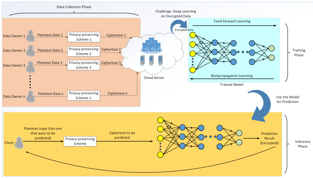
FIGURE 1. Illustration of PPDL Scheme
