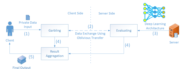
FIGURE 16. The Structure of Secure Two-party Computation-based PDDL
