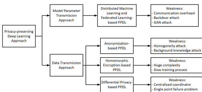
FIGURE 19. The Challenges and Weaknesses of State-of-the-Art PDDL Methods
