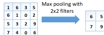
FIGURE 4. Pooling Layer
