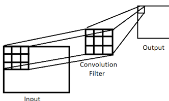
FIGURE 7. Convolutional Layer
