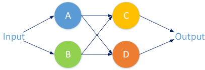
FIGURE 6. Dropout Layer
