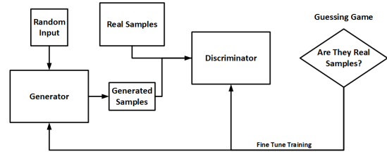
FIGURE 8. GAN Structure
