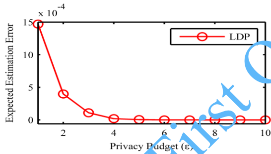
Figure 4. Expected estimation error curve using local differential privacy (LDP) for PPDAF.
