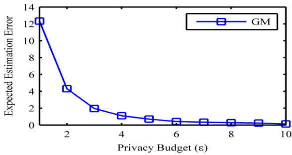
Figure 3. Expected estimation error curve using Gaussian mechanism (GM) for PPDAF.
