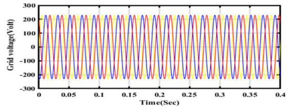
Figure 15 Grid voltage at I_{dref}=0 and I_{qref}=-5 with V_{dc}=300
