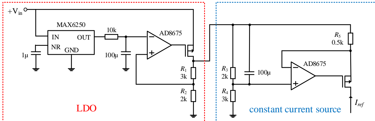
Fig. 2: Implementation of high-precision current reference I_{ref} . The low-dropout voltage regulator (LDO) uses a low-noise, precision voltage reference (MAX6250) with a 2 ppm/ ^{\circ}\text{C} temperature coefficient. Its output noise is further reduced by a low-pass filter, which attenuates noise frequencies above its 0.16 Hz cut-off frequency. The filtered reference voltage (5 V) is fed to the inverting terminal of a low noise, rail-to-rail operational amplifier (AD8675, Analog Devices), which regulates the output voltage through a p-channel power MOSFET and feedback resistors ( R_1 and R_2 ). The output voltage (12.5 V) serves as power supply for the high side current regulator. The voltage across R_3 sets the reference voltage that is forced across the current sense resistor R_5 by operational amplifier's negative feedback with unity gain. Thus, a constant current of 10 mA is generated.
