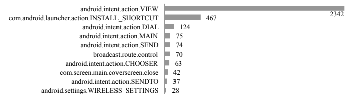
Fig. 21: Top 10 actions from Intents brought in rider code.
