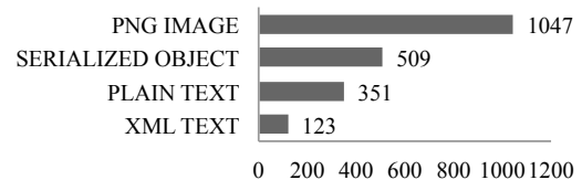
Fig. 11: Top types of resource files removed during piggybacking.
