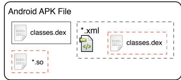
Fig. 2: An example of extra code of a given Android apps, where the extra code is highlighted with red dotted lines.
