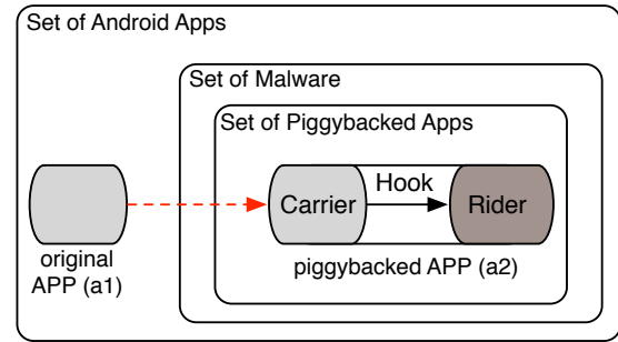
Fig. 1: Piggybacking terminology.
