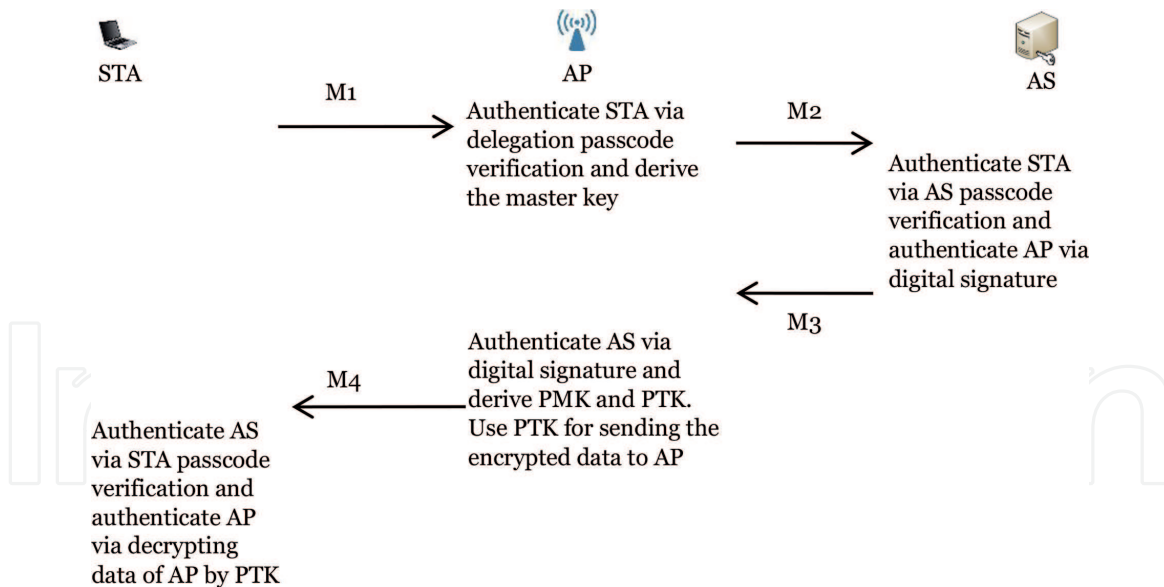
Figure 2. A simplified overview of online authentication phase of SWAS scheme.
