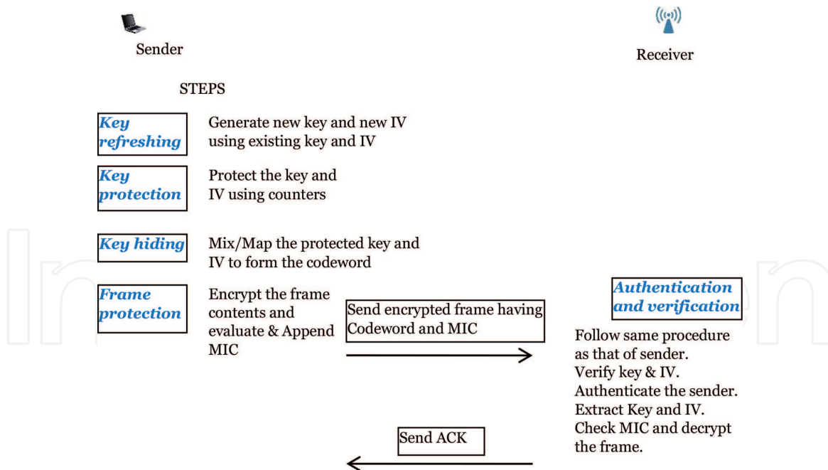
Figure 3. A simplified overview of communication phase of KHC scheme.
