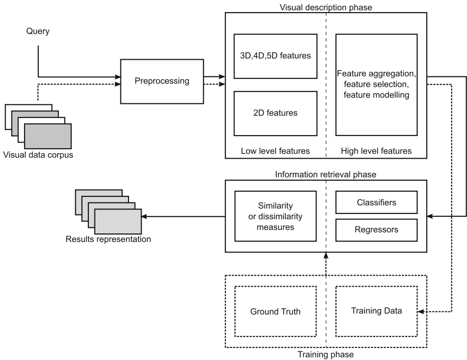
Fig. 7 Overview of a generic visual information retrieval system. The high-dimensional visual data from the retrieval corpus ( dashed line ) is processed and used as training data for supervised or unsupervised machine learning methods. The high-dimensional visual data from the query ( full line ) is processed in a similar way but is not involved in the learning process
