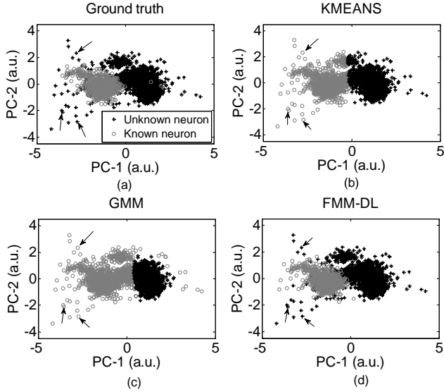
Fig. 2. Clustering results shown in the 2 PC space of the various methods on d533101 data [17]. All abbreviations are explained in the main text (Section III-A). “Known neuron” denotes waveforms associated with the neuron from the cell with the intracellular recording, and “Unknown neuron” refers to all other detected waveforms. Note that all methods are shown in the first two PCs for visualization, but that the FMM-DL shown in (d) is jointly learning the feature space and clustering.
