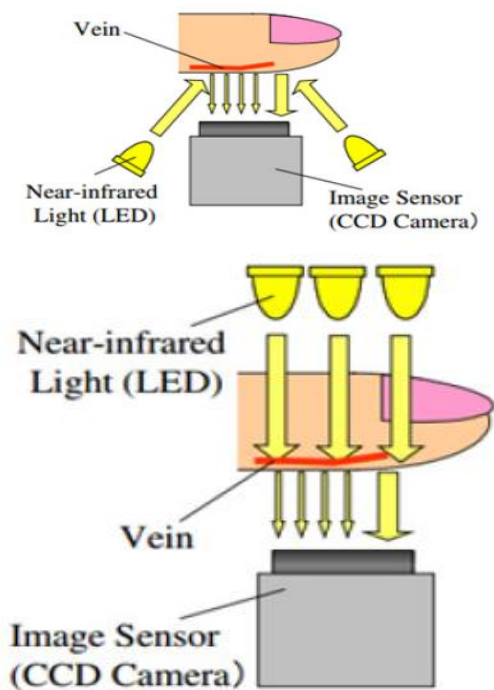
Figure.6 Two ways of finger vein image acquisition
