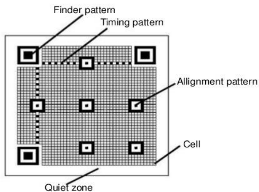
Fig 1. Structure of QR code
