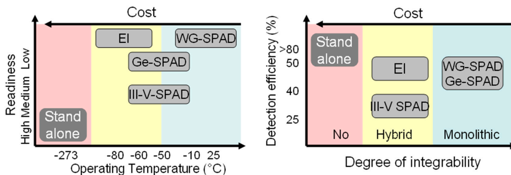
Figure 2. Quantum detector overview. (WG-SPAD = waveguide single-photon avalanche diodes).
