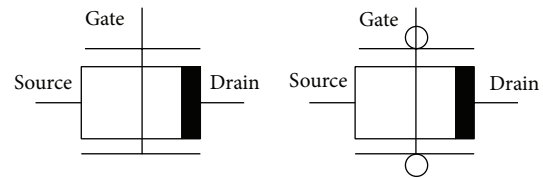
FIGURE 10: Asymmetric drain-source doped (AD) FinFET [58].
