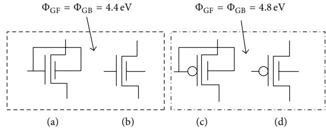
FIGURE 16: Schematic diagrams of (a) SG nFinFET, (b) IG nFinFET, (c) SG pFinFET, and (d) IG pFinFET. Their gate workfunctions are also shown [49].
