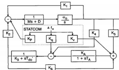
Fig. 2 Phillips- Heffron model of a single machine infinite-bus power system installed with a STATCOM
