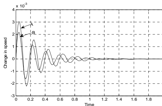
Fig. 11 Dynamic response of \Delta\omega for STATCOM with additional power oscillation damping controller for different values of X_e a) X_e=0.3 b) X_e=0.65
